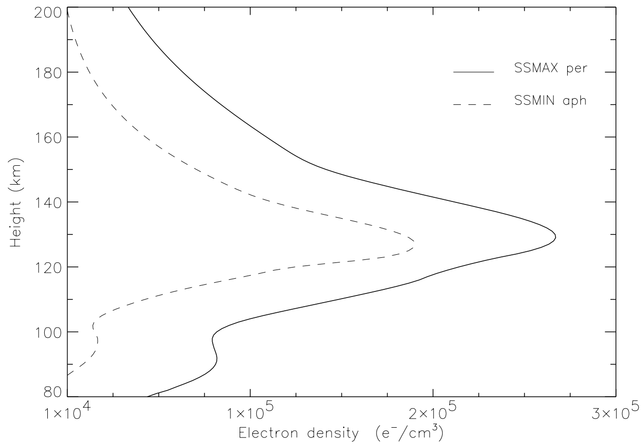
Figure 10. Model results showing N_e(h) profile shape changes at the sub-solar point for the extreme cases of Mars at aphelion at solar minimum versus perihelion at solar maximum.
