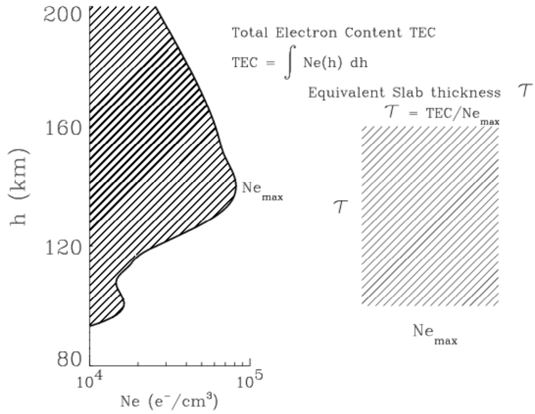
Figure 7. Illustration of three parameters used to characterize an ionospheric N_e(h) profile: N_{\text{max}} , TEC and equivalent slab thickness \tau .
